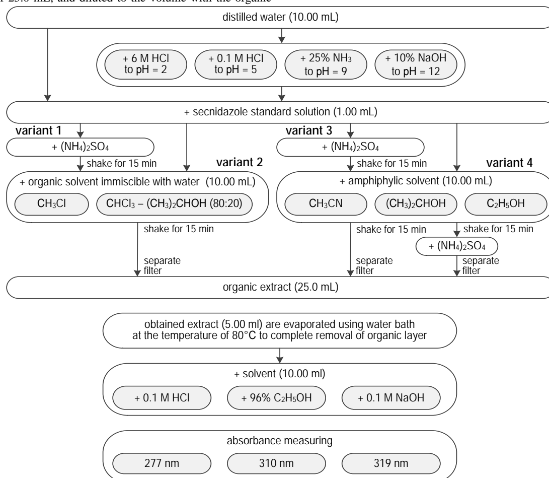
Scheme 1. The main stages of secnidazole extraction procedures
